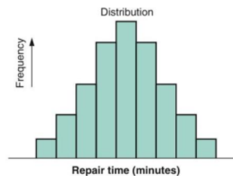
Gambar 5 Histogram
